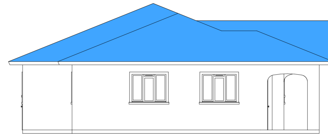
ELEVATION 03
