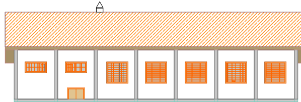
NORTH ELEVATION
