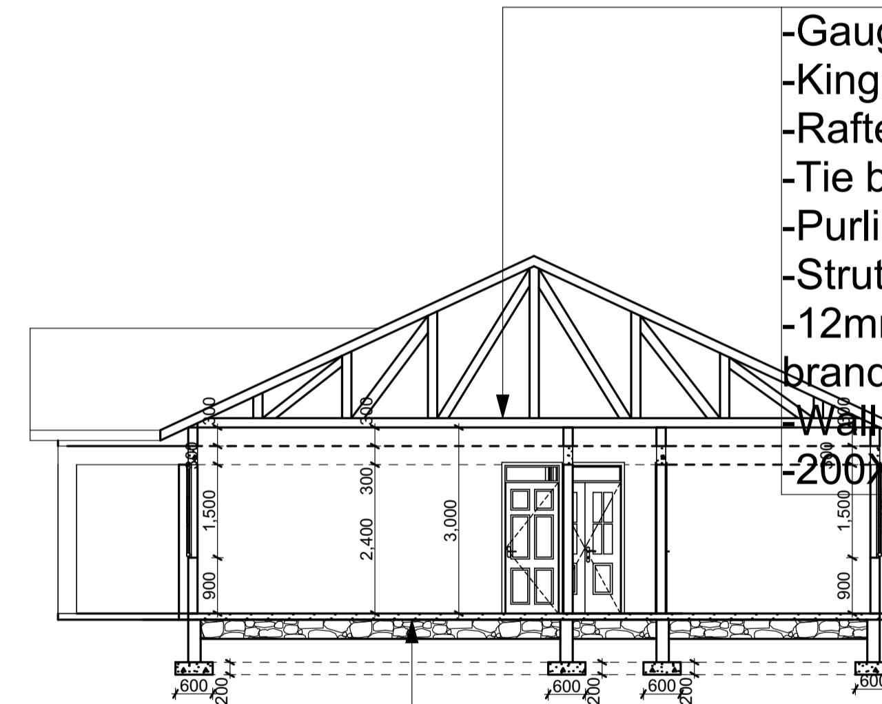
Sub structure section
