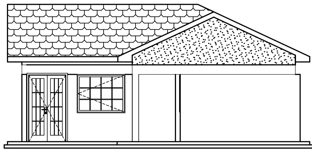
Front(01)Elevation
