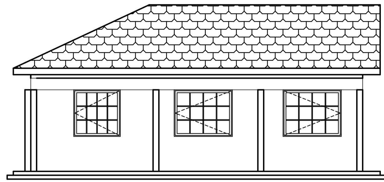
Rear(02)Elevation
