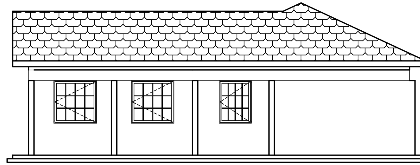
Side(03)Elevation
