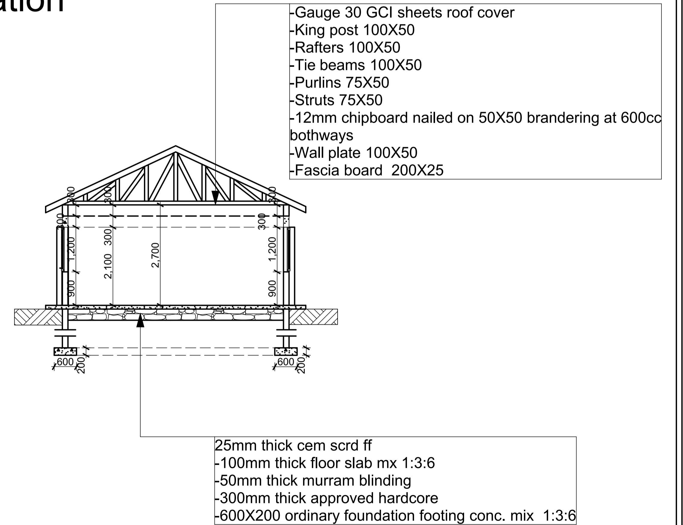
Cross section S-01<->S-01
