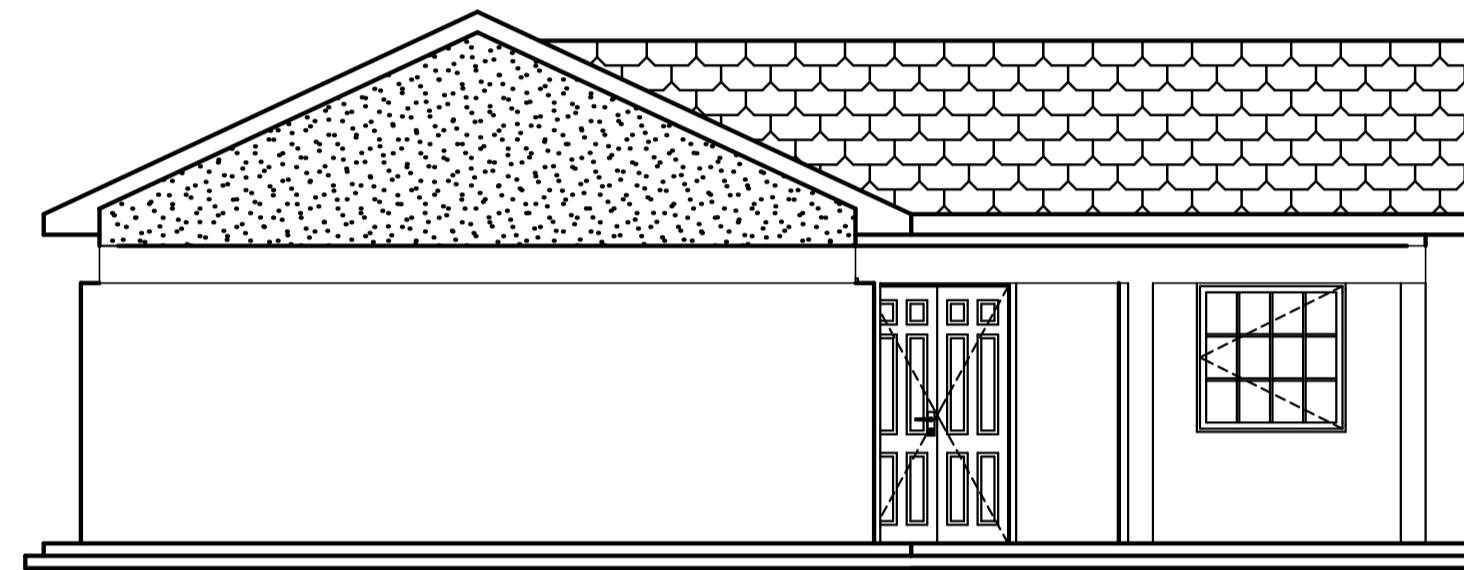
Side(04)Elevation
