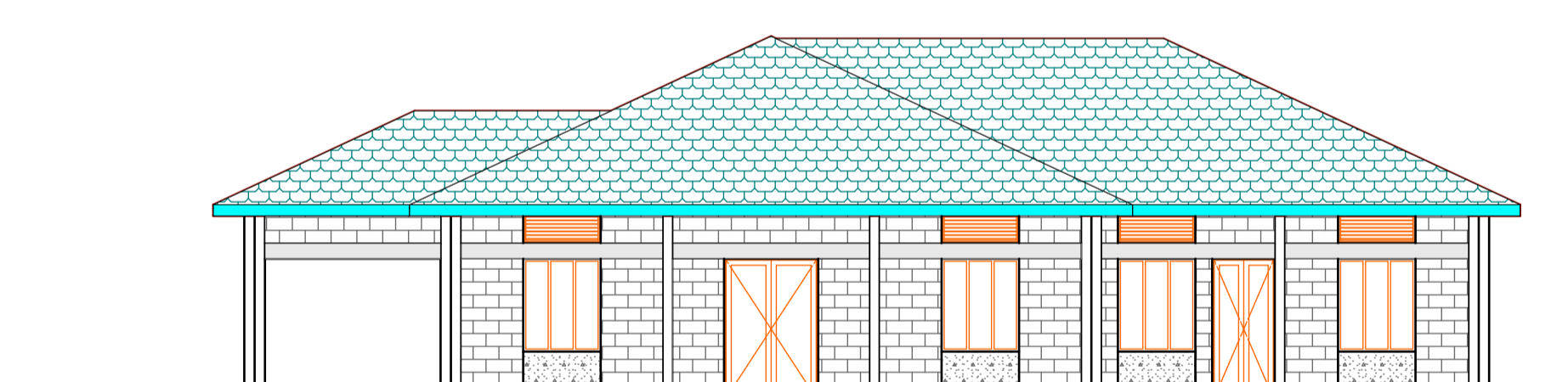
SIDE ELEVATION 04.
