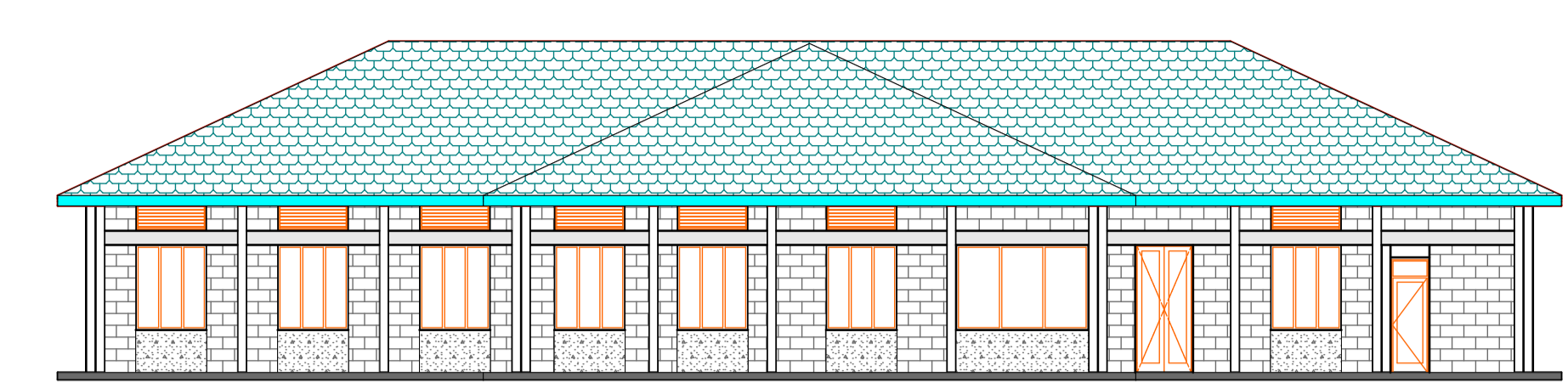
REAR ELEVATION 01.
