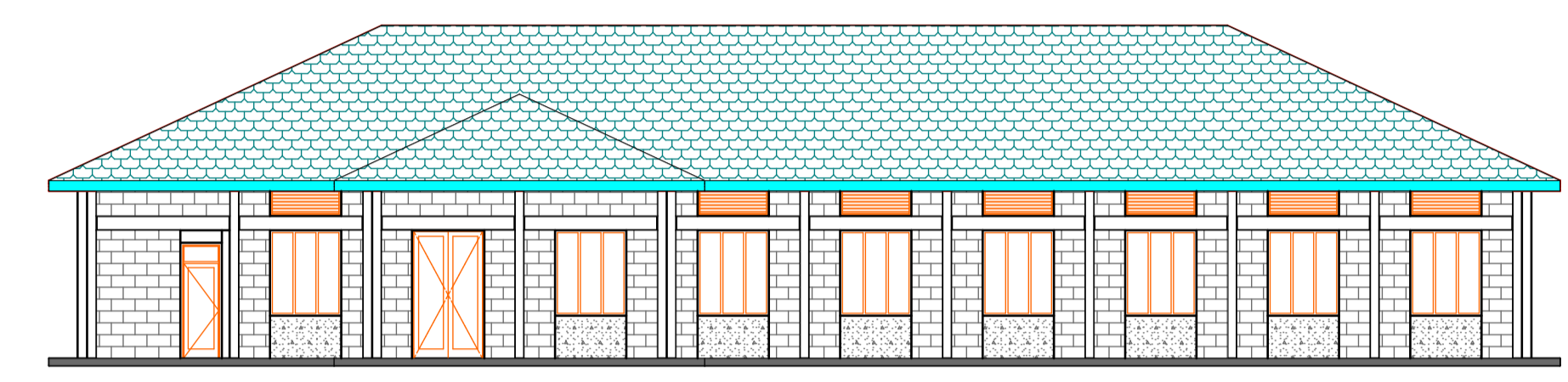
FRONT ELEVATION 03.
